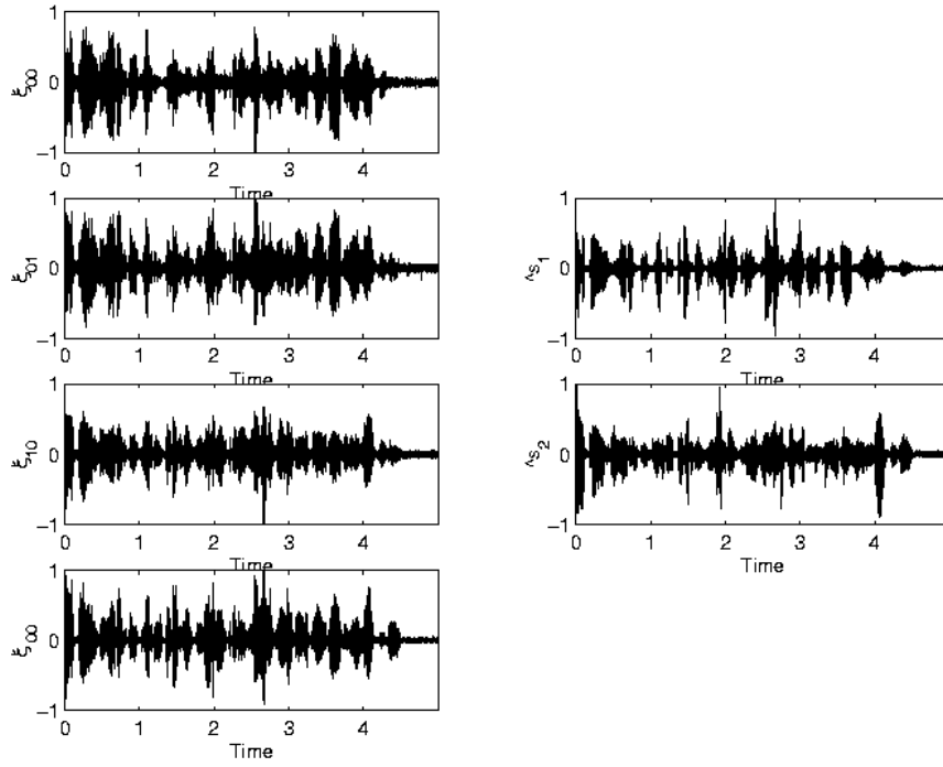
Fig. 4. Experimental separation of speech from two male speakers in an outdoors setting. Left: Measured components \xi_{00} , \xi_{10} , \xi_{01} and its time derivative \xi_{00} , produced by the analog circuit in Fig. 3 on outputs from the microphone array in Fig. 1. Right: Reconstructed sources \hat{s}_1 and \hat{s}_2 using static ICA on \xi_{10} , \xi_{01} and \xi_{00} .
