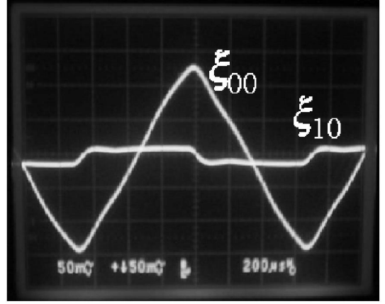
Fig. 2. Common-mode \xi_{00} and gradient \xi_{10} components obtained from the microphone array of Fig. 1, for a single audio signal generated from a triangular waveform source. \xi_{10} approximates the time derivative \dot{\xi}_{00} , scaled by the angle cosine \tau_1 in all four quadrants.
