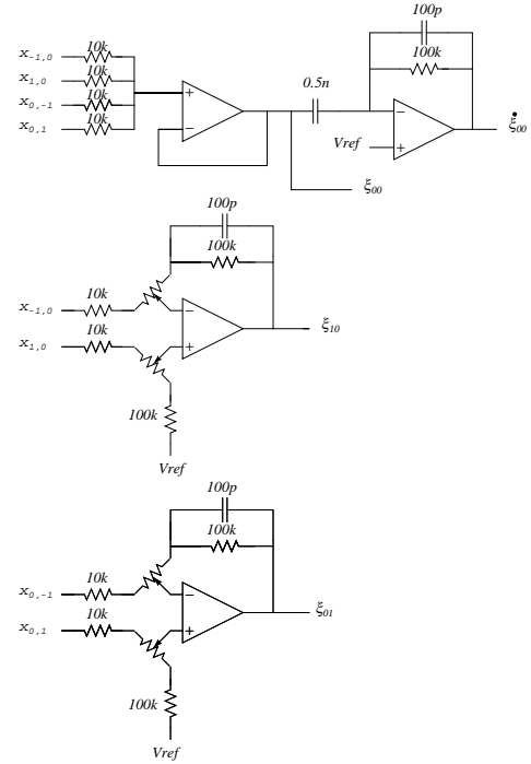
Fig. 3. Analog circuit computing common-mode \xi_{00} , spatial derivatives \xi_{10} and \xi_{01} , and the common-mode time derivative \dot{\xi}_{00}
