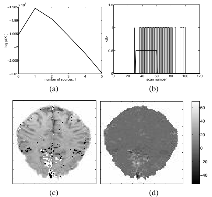
Fig. 1. Analysis of a fMRI data set using temporal binary ICA. (a) shows the log marginal likelihood as a function of the number of hidden sources. At l = 0 the log marginal likelihood is calculated for a Gaussian with common variance. (b) shows the experimental paradigm (in solid) and the inferred sources. (c) shows the .025 (black) and .975 (white) fractiles of the values in the eigenimage superimposed on an anatomical reference. (d) shows a quantitative representation of the spatial pattern retaining only the 0.1 and 0.9 fractiles of the eigenimage.
